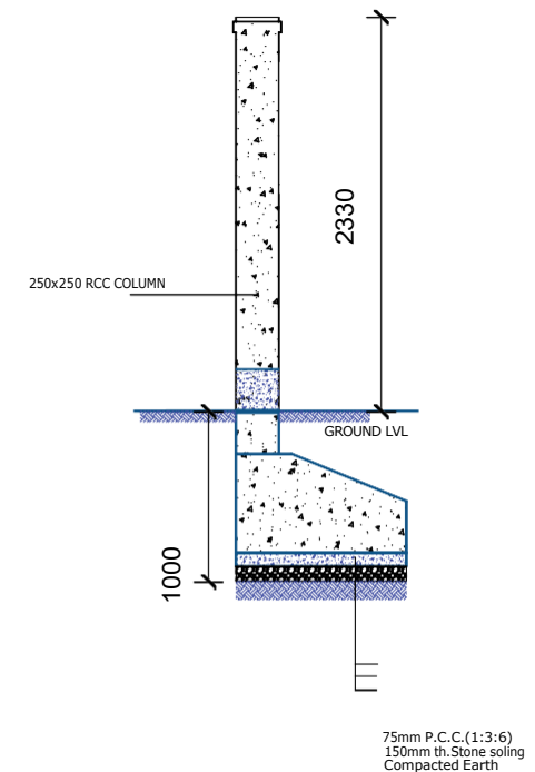
TYPICAL CROSS SECTION OF WALL AT B-B
