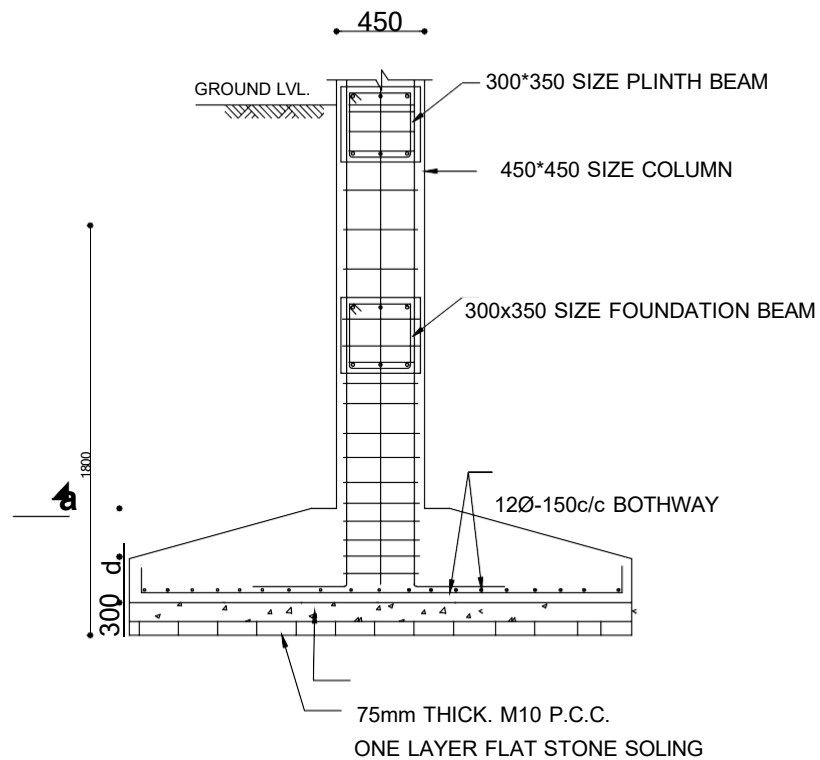
MAIN GATE FOOTING SECTION
